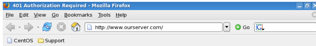
Figure 49: Authorization required
