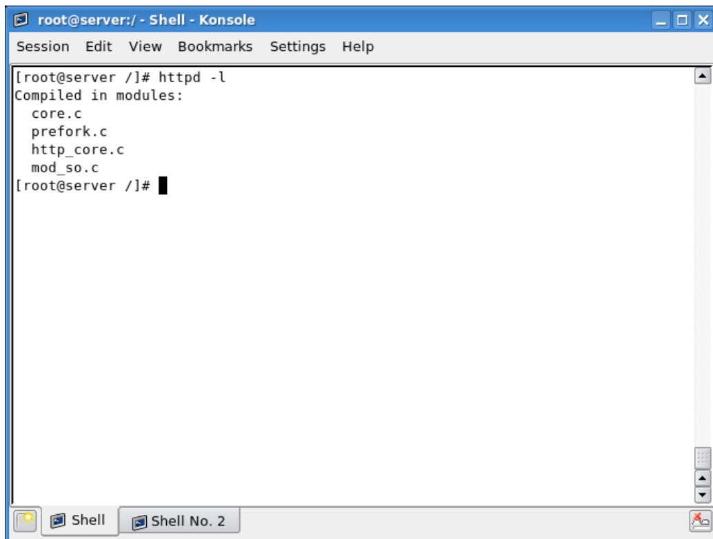
Figure 39: Listing compiled modules
