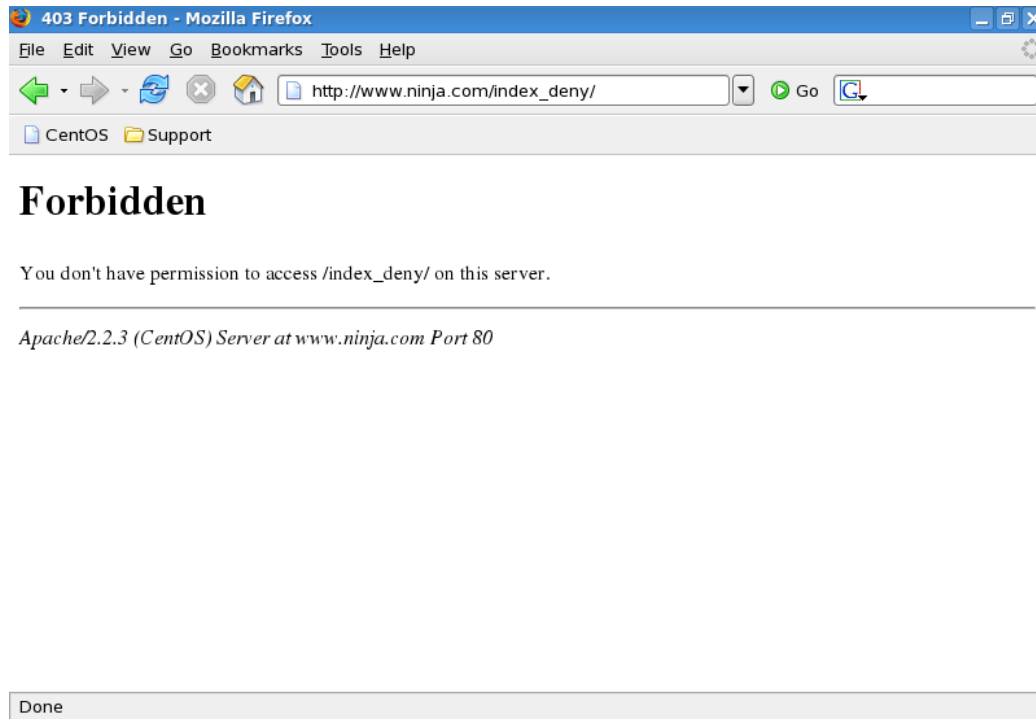
Figure 25: index_deny example
